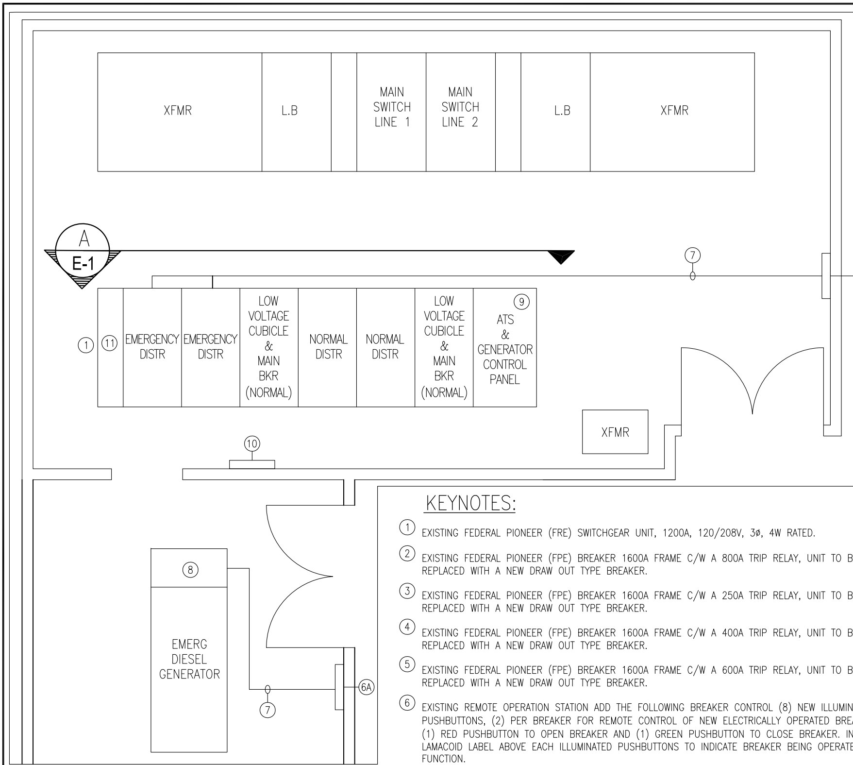
MAIN ELECTRICAL ROOM LAYOUT
